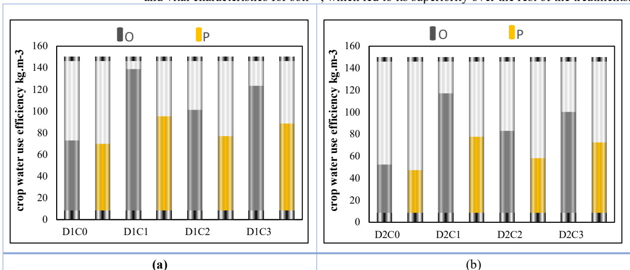
Figure 6. Crop water use efficiency that simulated under natural conditions for the different study treatments.
